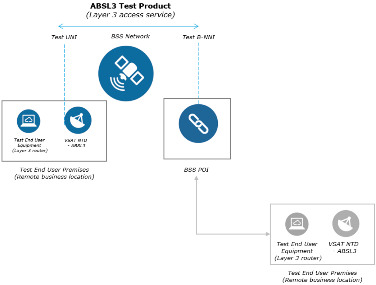
Figure A4: ABSL3 Test Product (Test UNI to Test UNI configuration)
