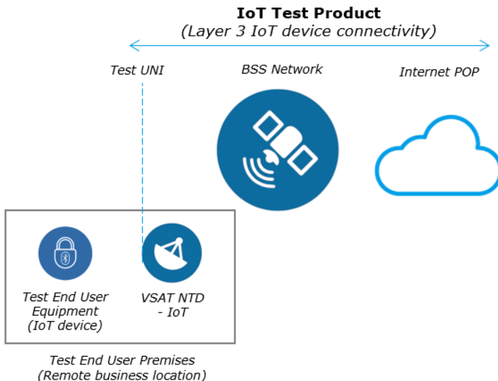
Figure A2: IoT Test Product
