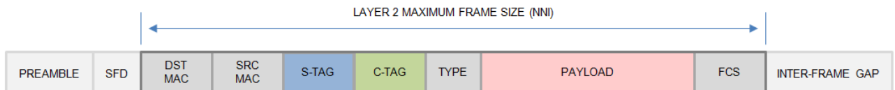
Figure 10 Definition of Maximum Layer 2 Frame Size (NNI)
