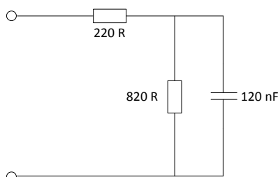
Figure 5 - TN12 impedance
