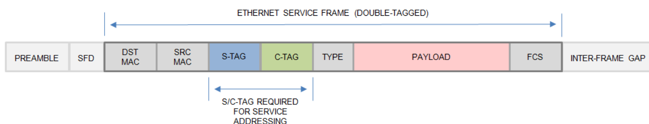
Figure 2 Service Addressing Mode A Frame Format 3
